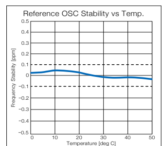
TCXO temperature drift characteristics ●Values are measured examples.
