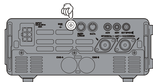
Improper Ground Connection
